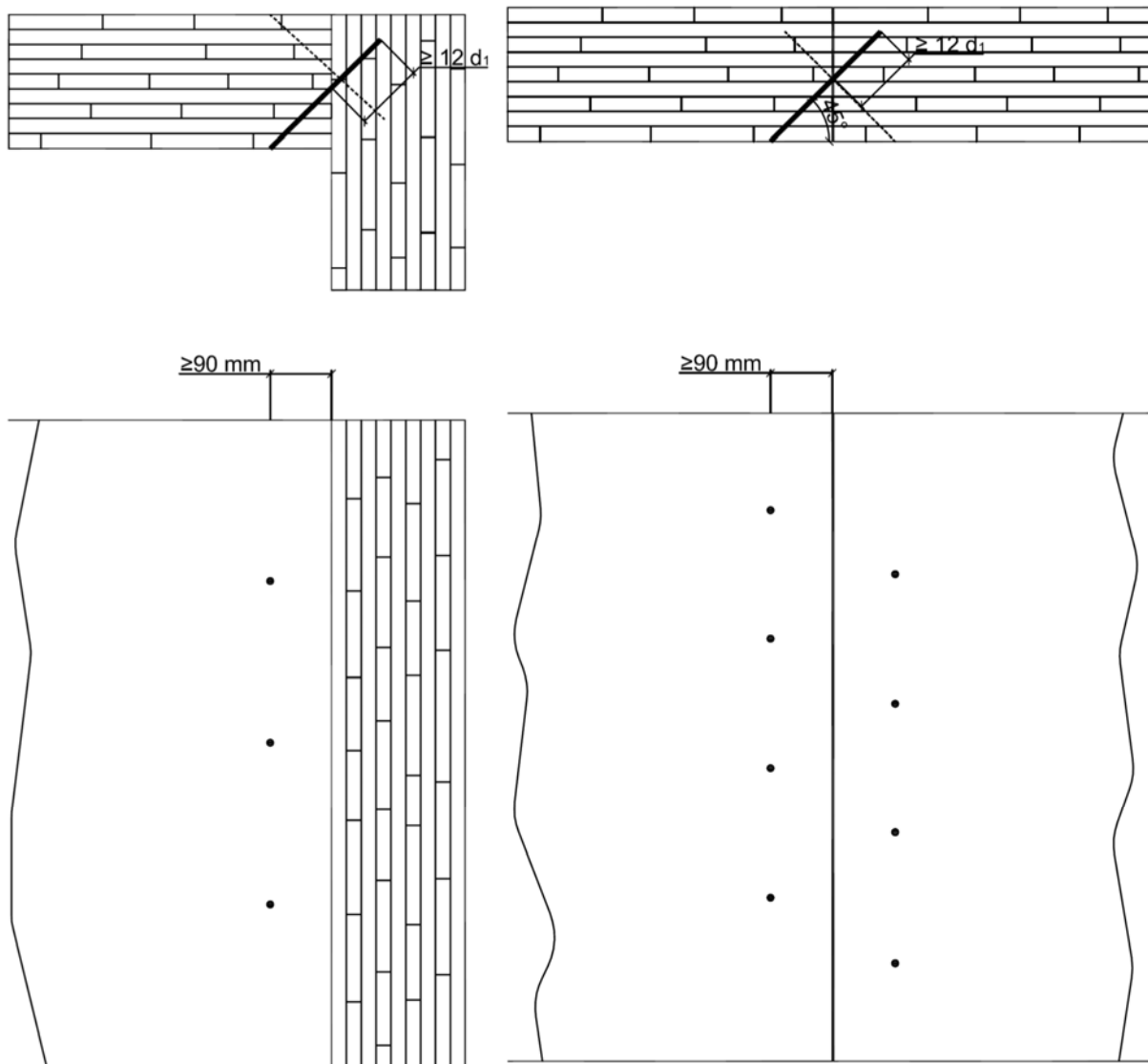
Figure 8: Perpendicular and parallel connection of MHM – wall elements
