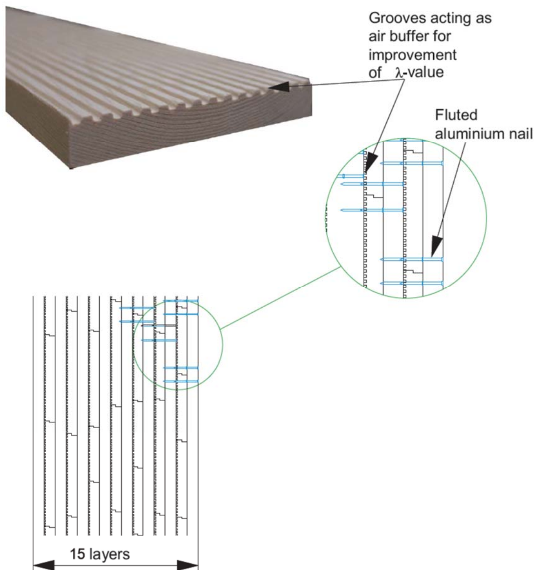
Figure 3: Principle structure of the MHM – wall element with grooved board layers
